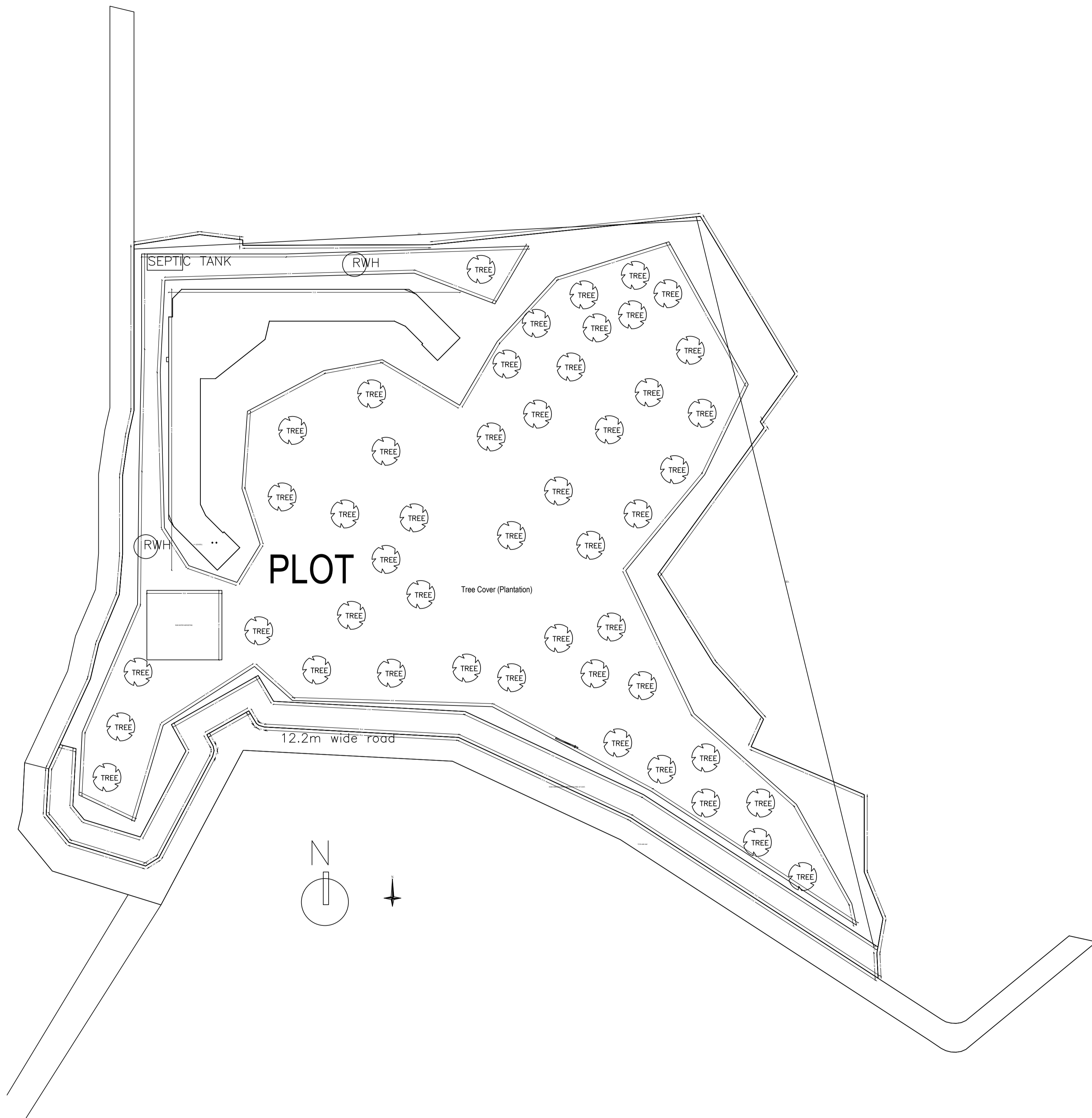
SITE PLAN
