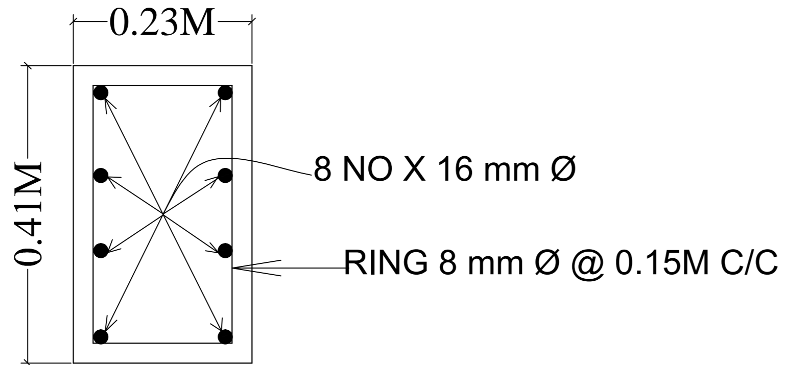
C.S. OF COLUMN . SIZE - 0.23M X 0.41M
