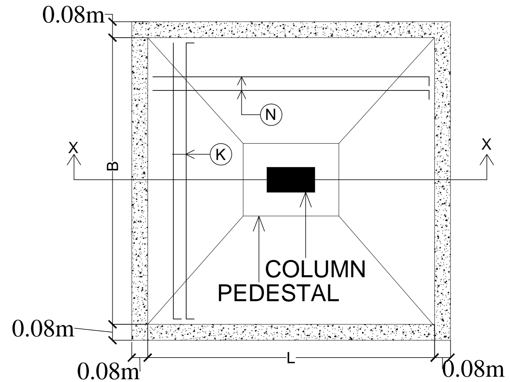
PLAN OF ISOLATED FOOTING
