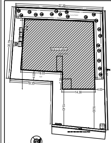
SITE PLAN
