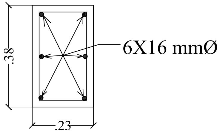
SECTION OF COLUMN. - C1
