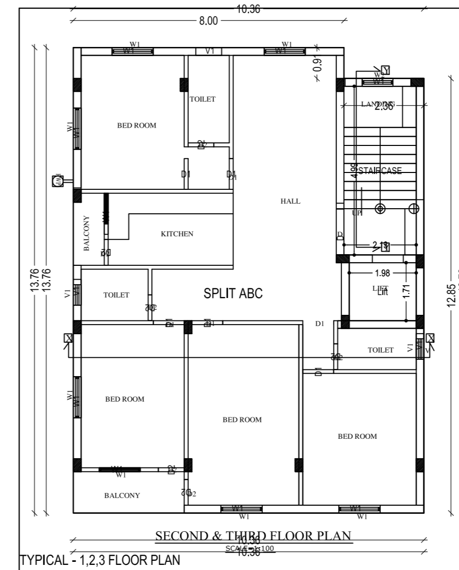
TYPICAL - 1,2,3 FLOOR PLAN
