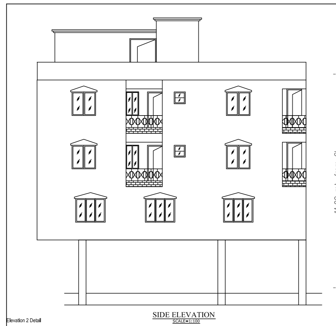
Elevation 2 Detail
