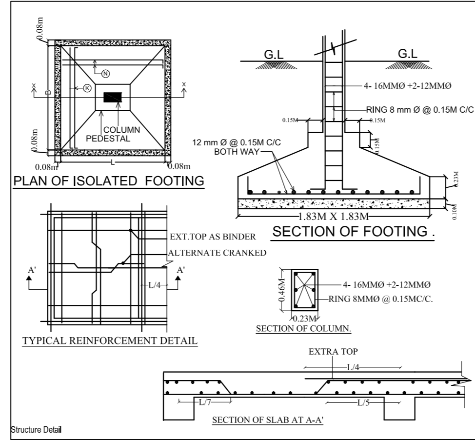
Structure Detail
