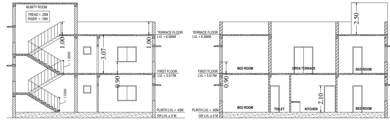
SECTION - XX scale - 1:100
