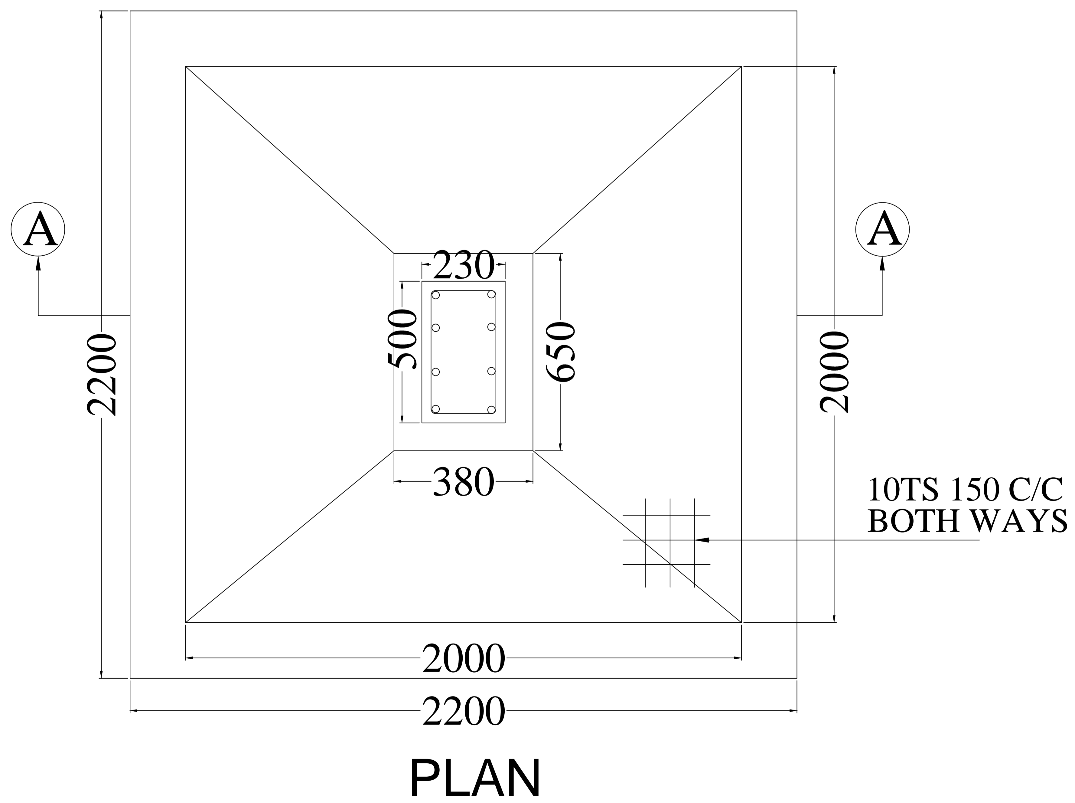
FOOTING PLAN (AS/STRL. DESIGN) SCALE N.T.S
