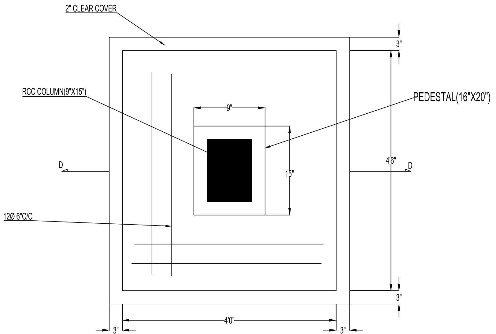
FOOTING-F1
