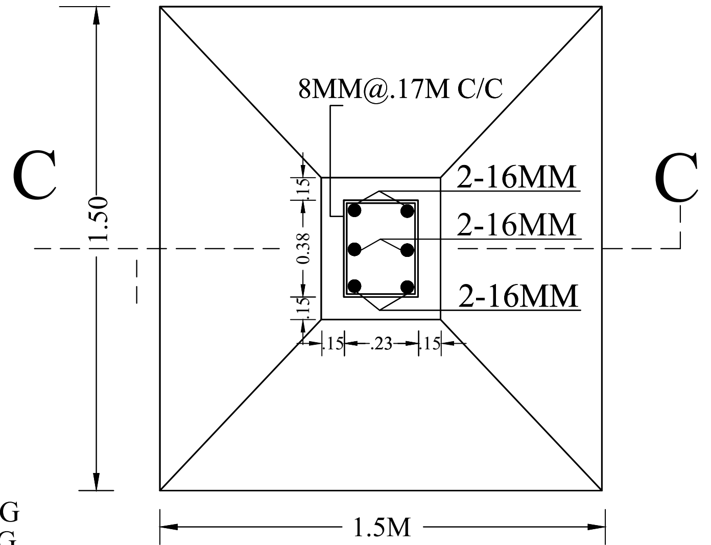
R.C.C. COL. FDN. PLAN SCALE -1:25
