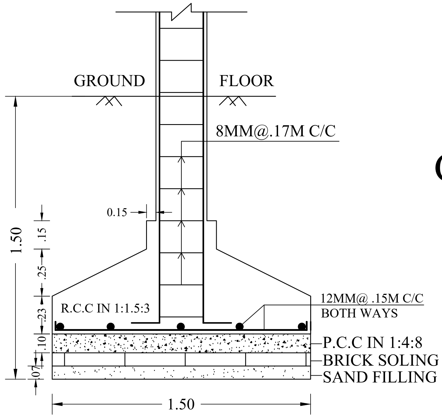
SECTION - CC SCALE -1:25
