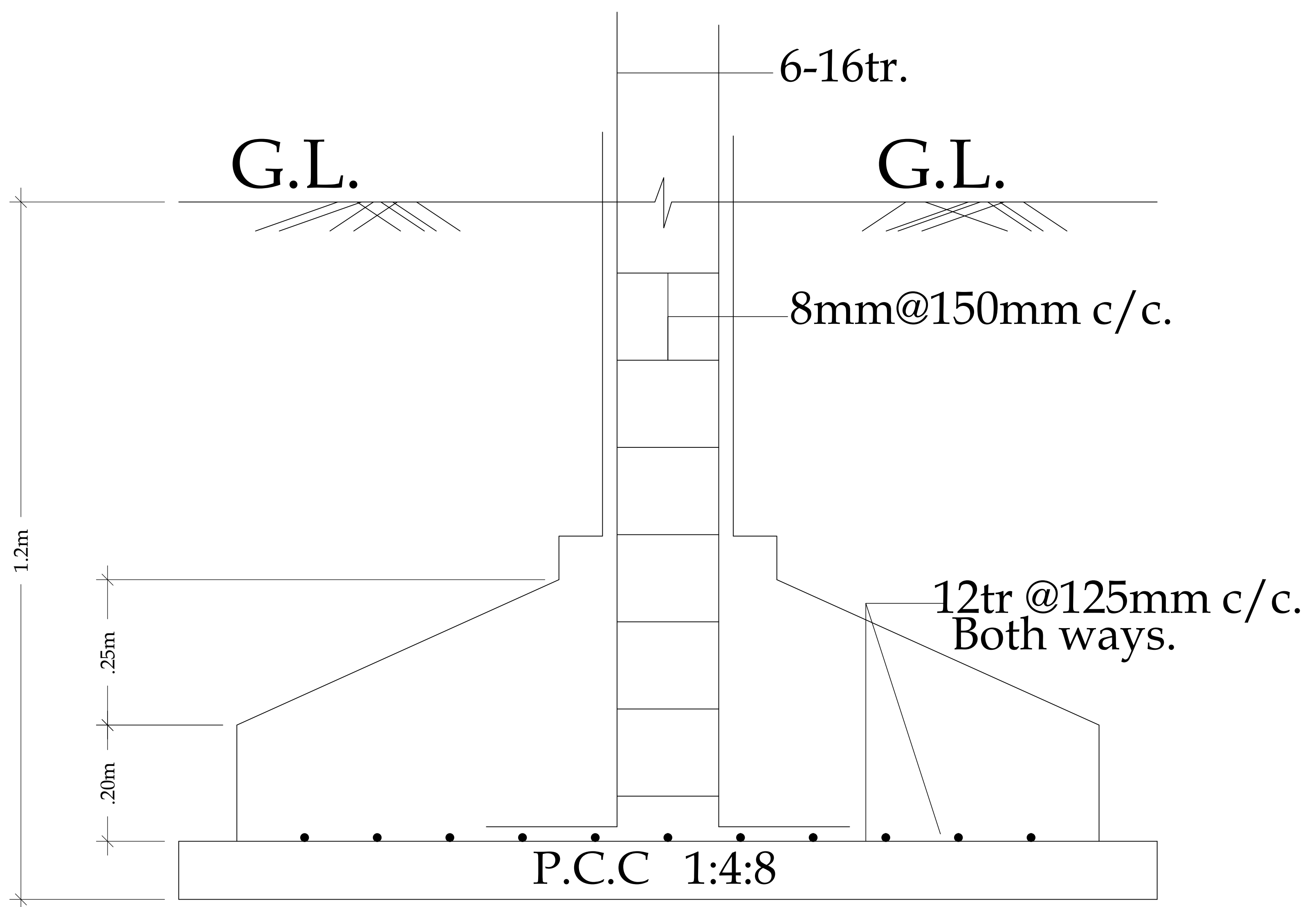
SECTION ON = X-X
