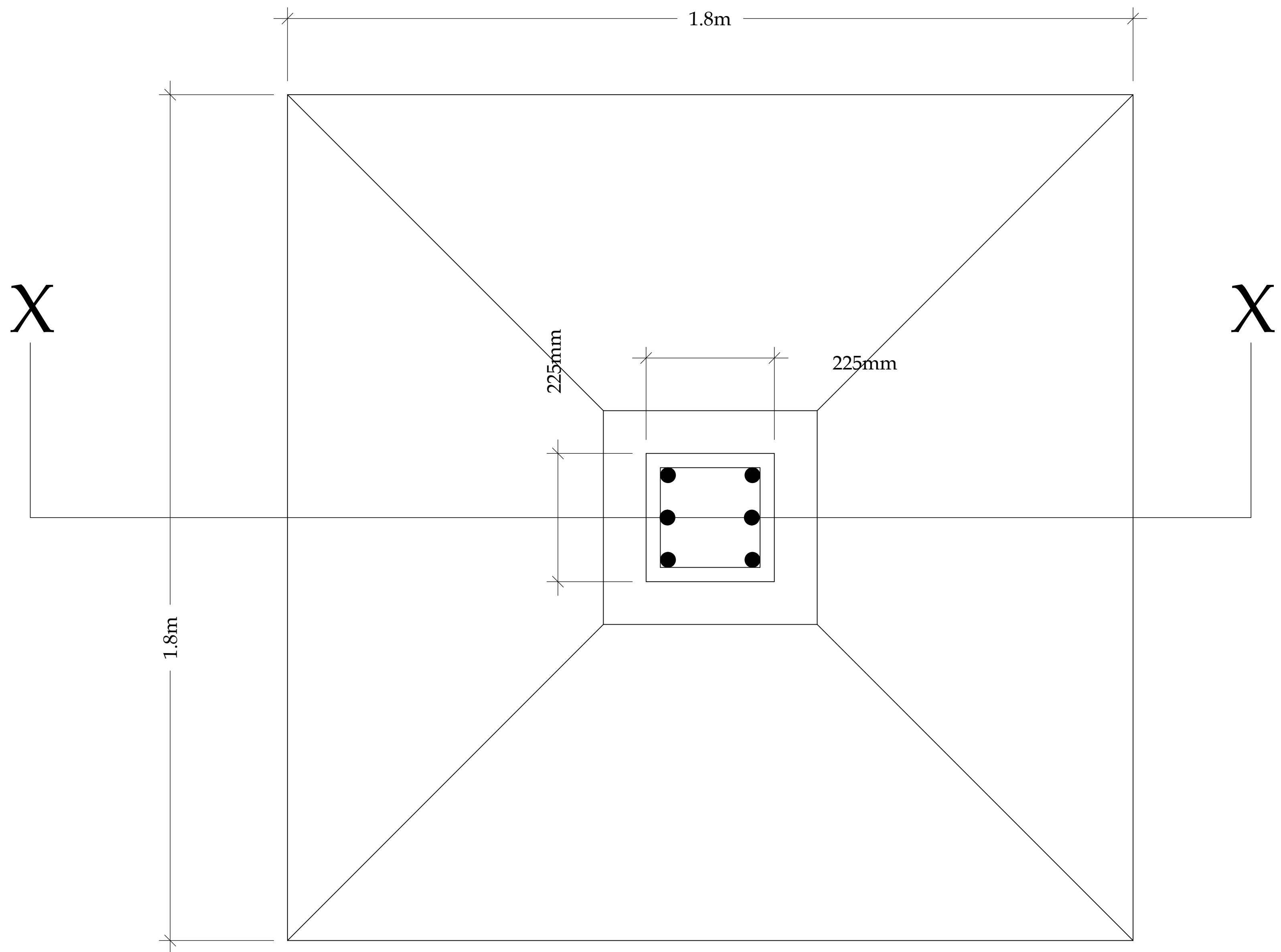
DETAIL OF FOOTING (Not to Scale)
