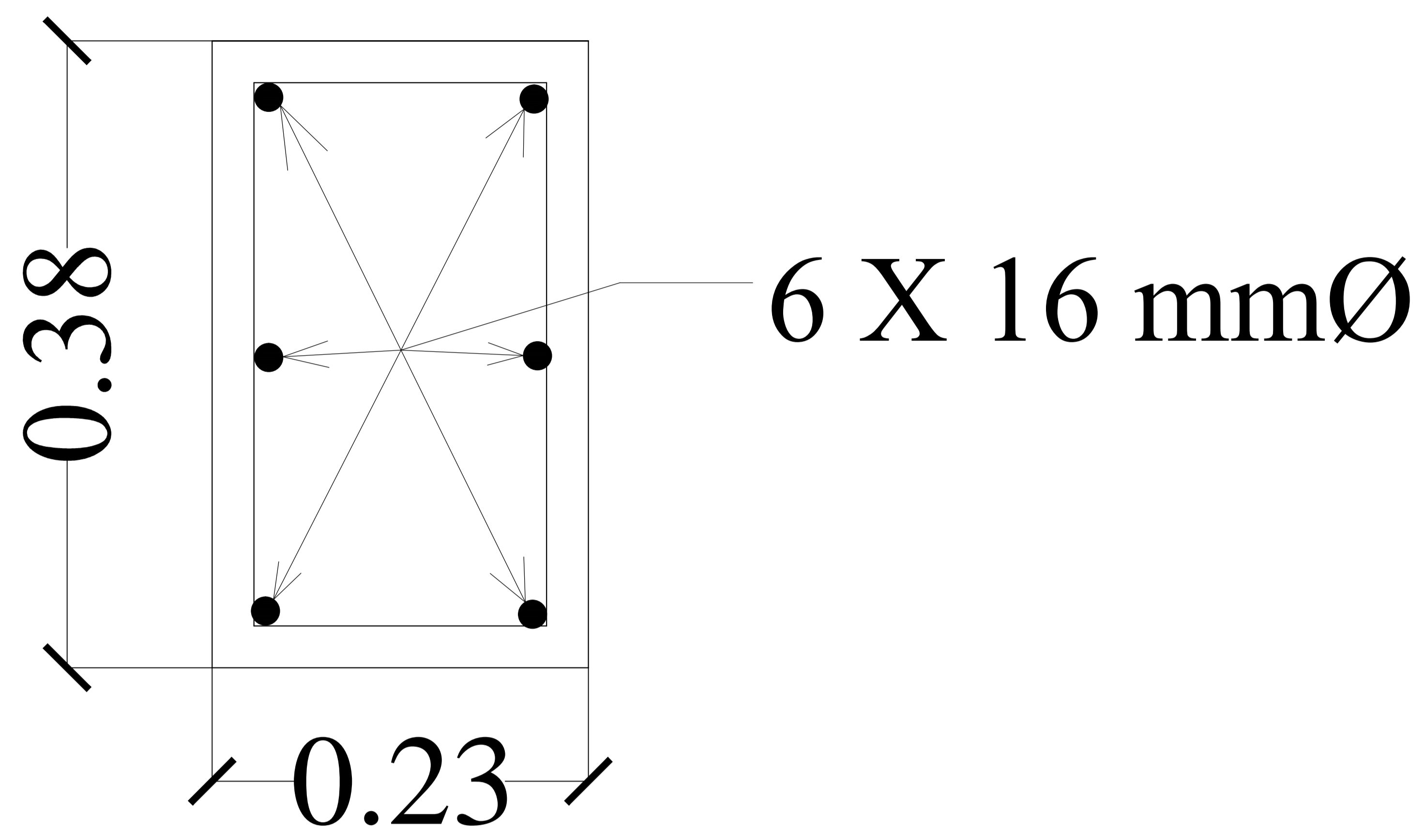
SECTION OF COLUMN.
