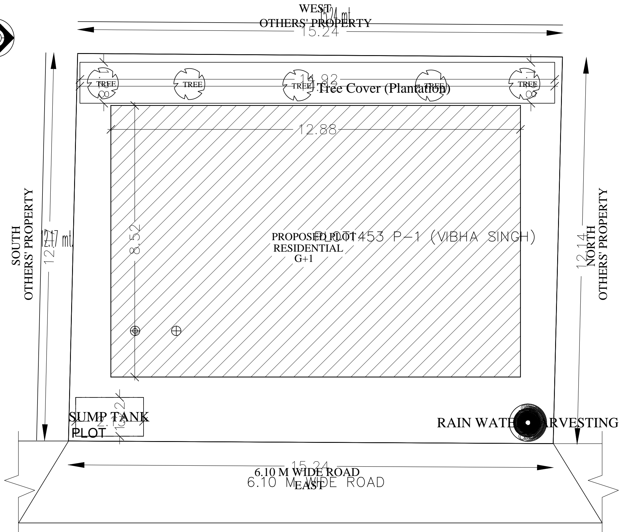
SITE PLAN
