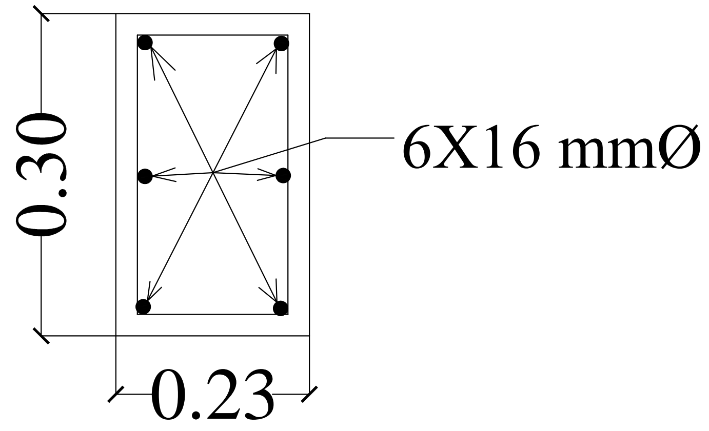
SECTION OF COLUMN
