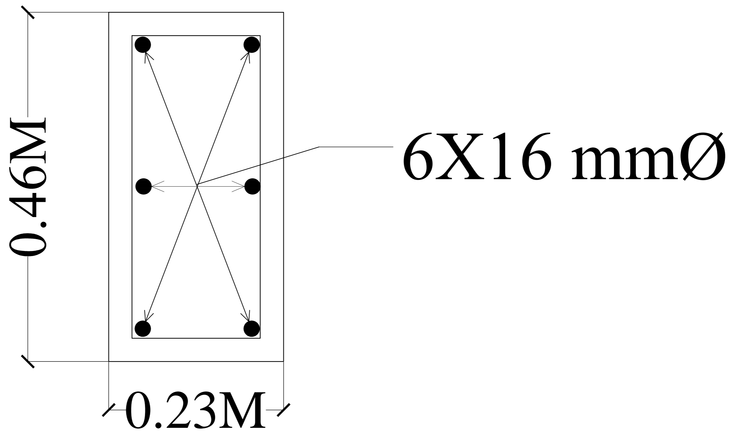
SECTION OF COLUMN.
