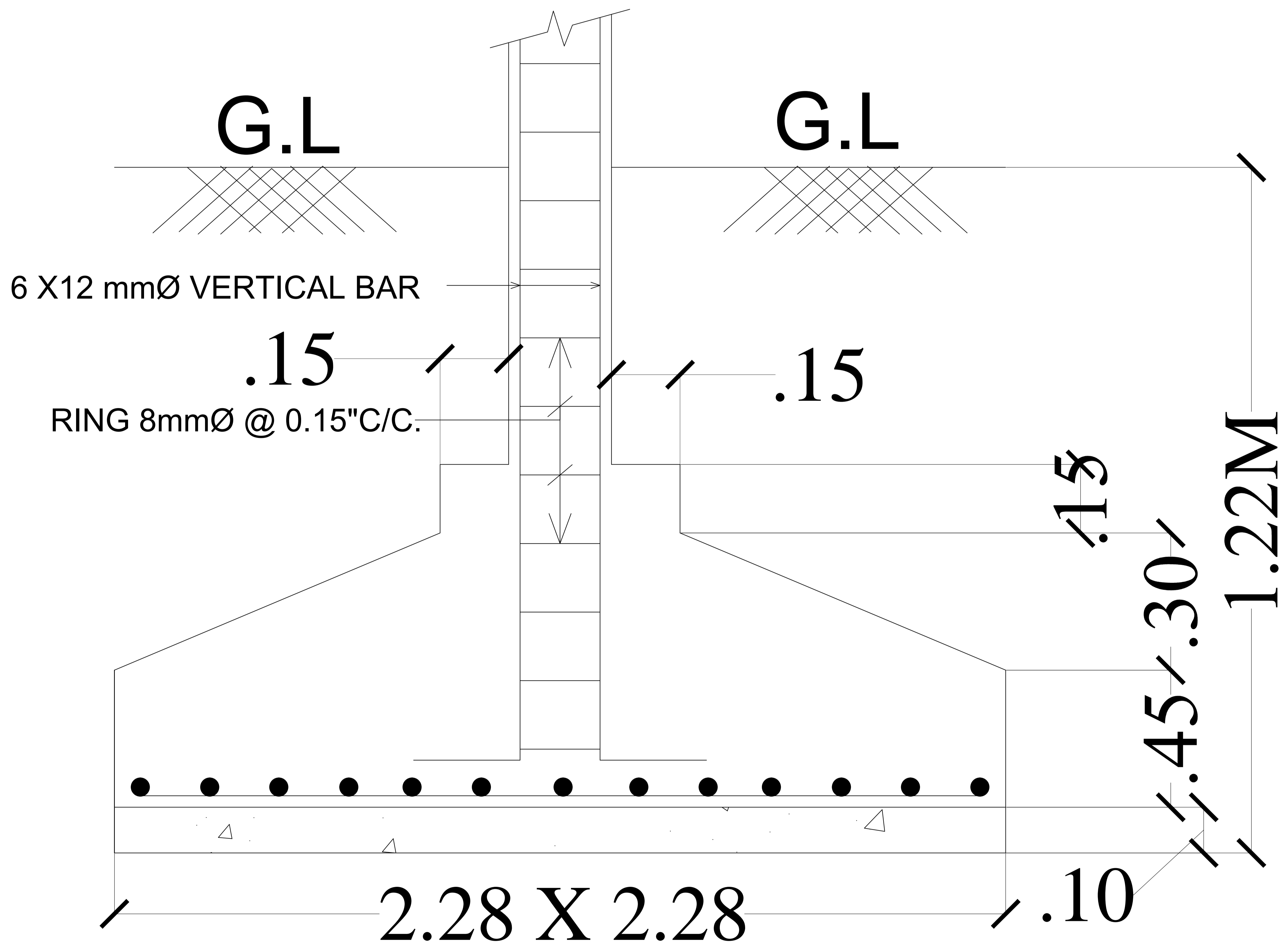
SECTION OF FOOTING
