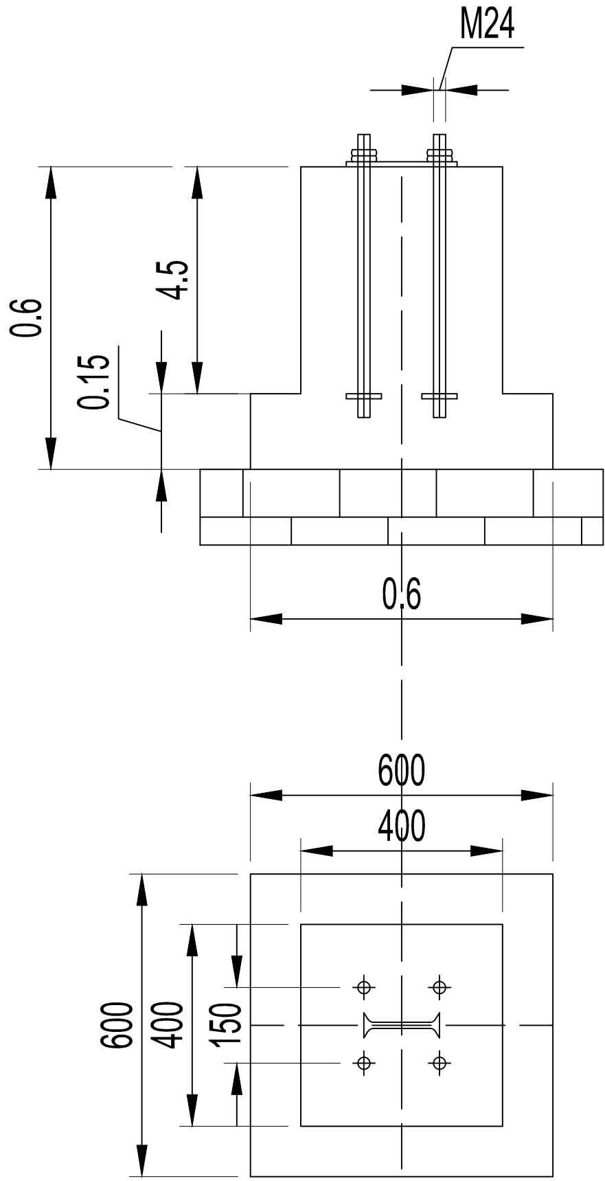
FOUNDATION DETAILS OF STRUCTURE
