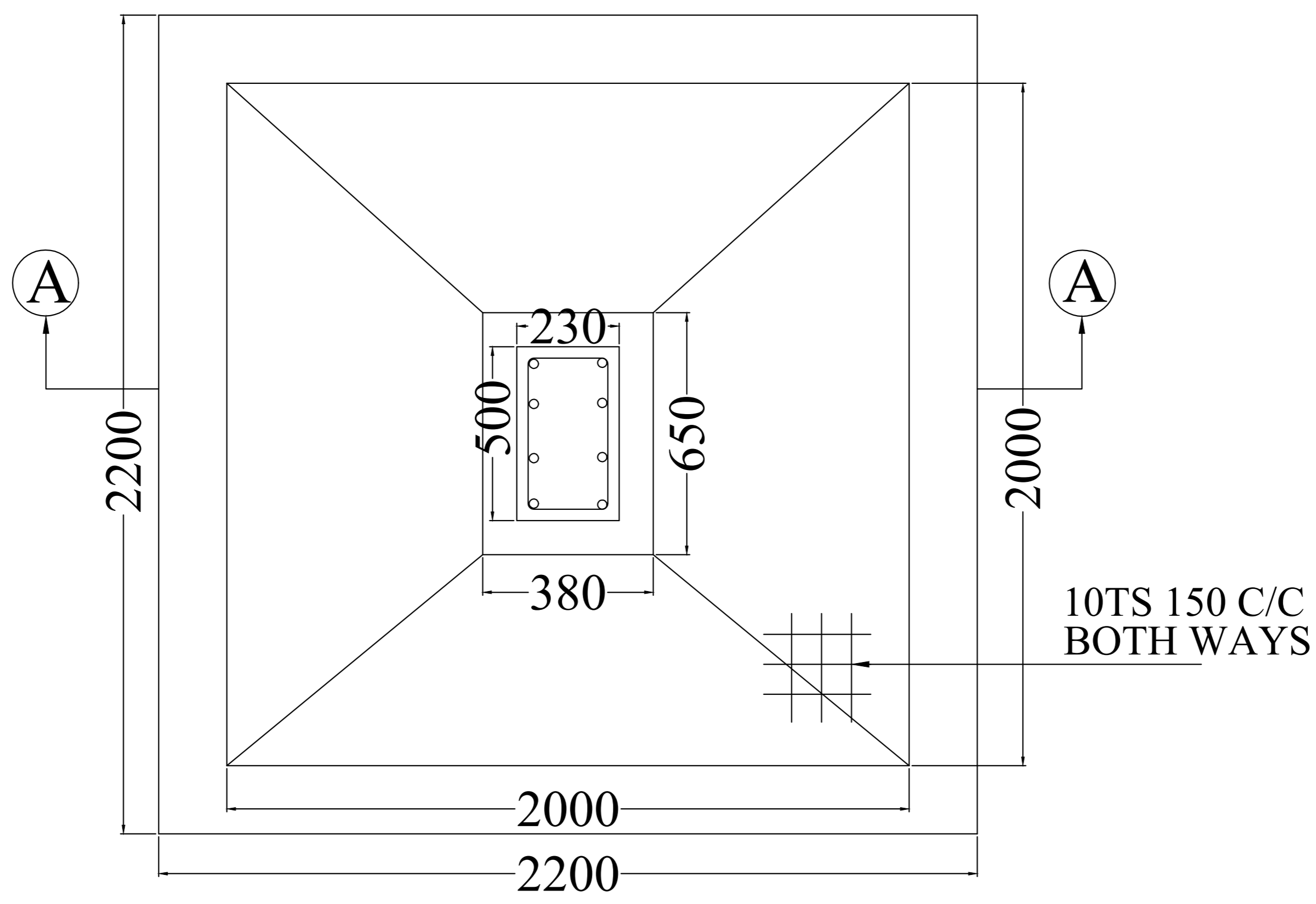
PLAN
