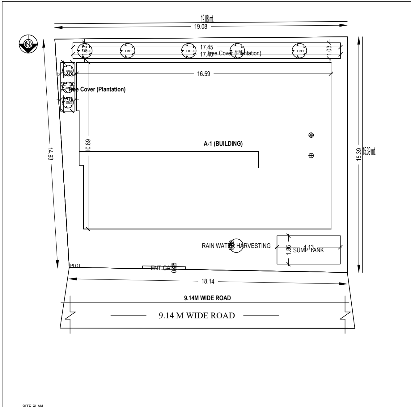
SITE PLAN
