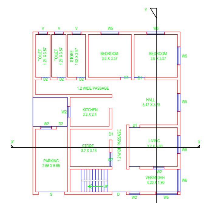
EXISTING GROUND FLOOR PLAN SCALE : 1:100
