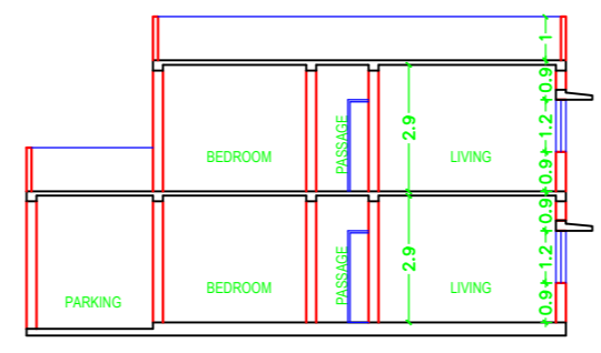
SECTION -Y-Y' SCALE : 1:100
