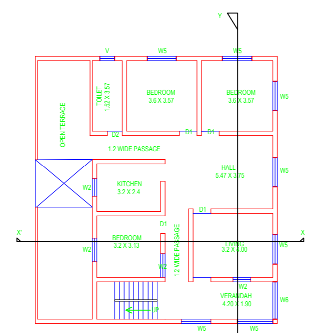
EXISTING 1ST FLOOR PLAN SCALE : 1:100
