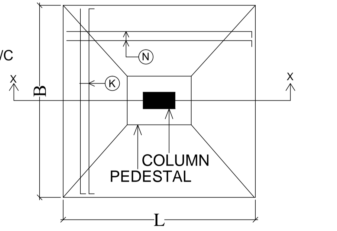
PLAN OF ISOLATED FOOTING
