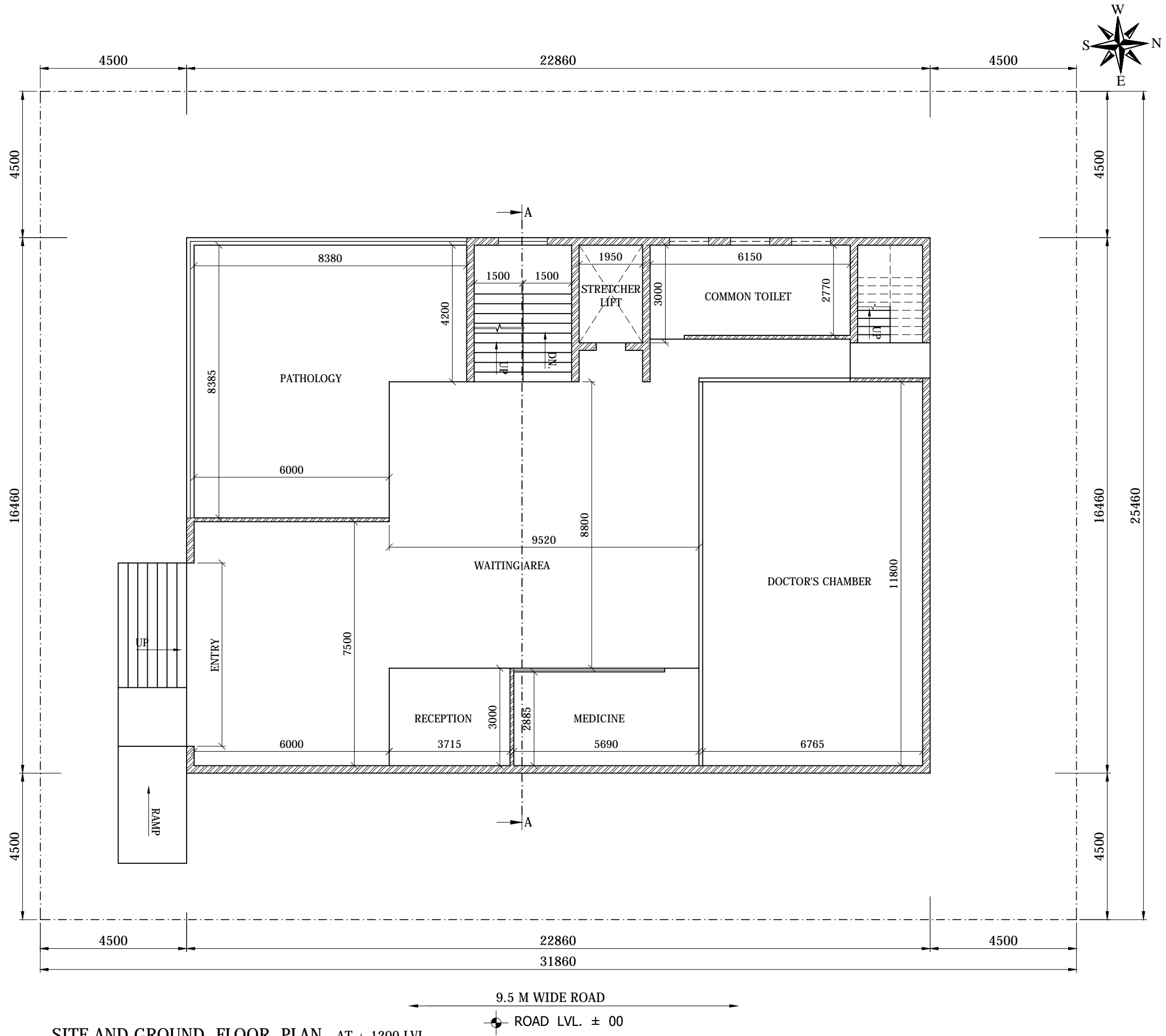
SITE AND GROUND FLOOR PLAN AT + 1200 LVL.
