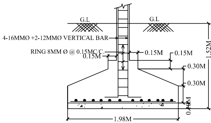
SECTION OF FOOTING
