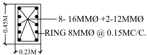
SECTION OF COLUMN.
