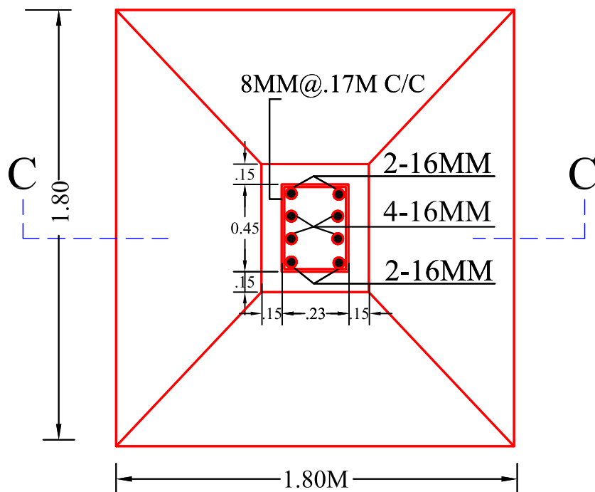
R.C.C. COL. FDN. PLAN SCALE -1:25
