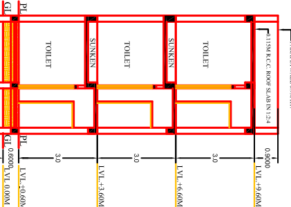
SECTION-BB SCALE 1:100
