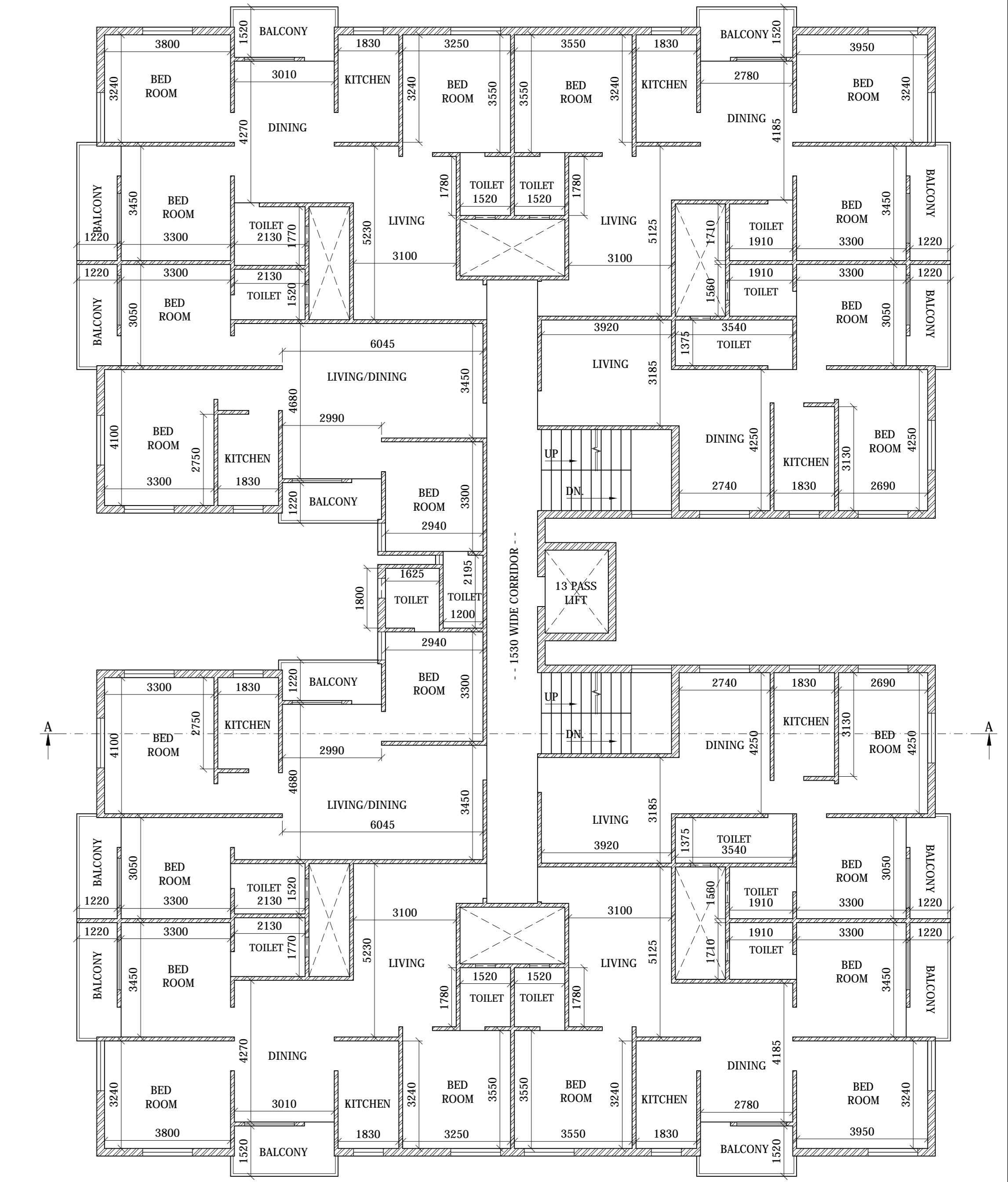
TYPICAL SECOND, THIRD & FOURTH FLOOR PLAN
