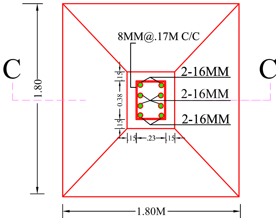
R.C.C. COL. FDN. PLAN SCALE -1:25
