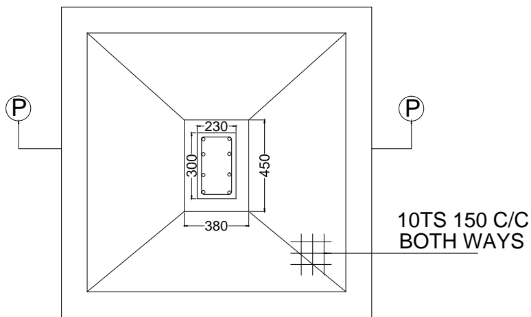
PLAN FOOTING PLAN (AS/STRL. DESIGN) SCALE N.T.S
