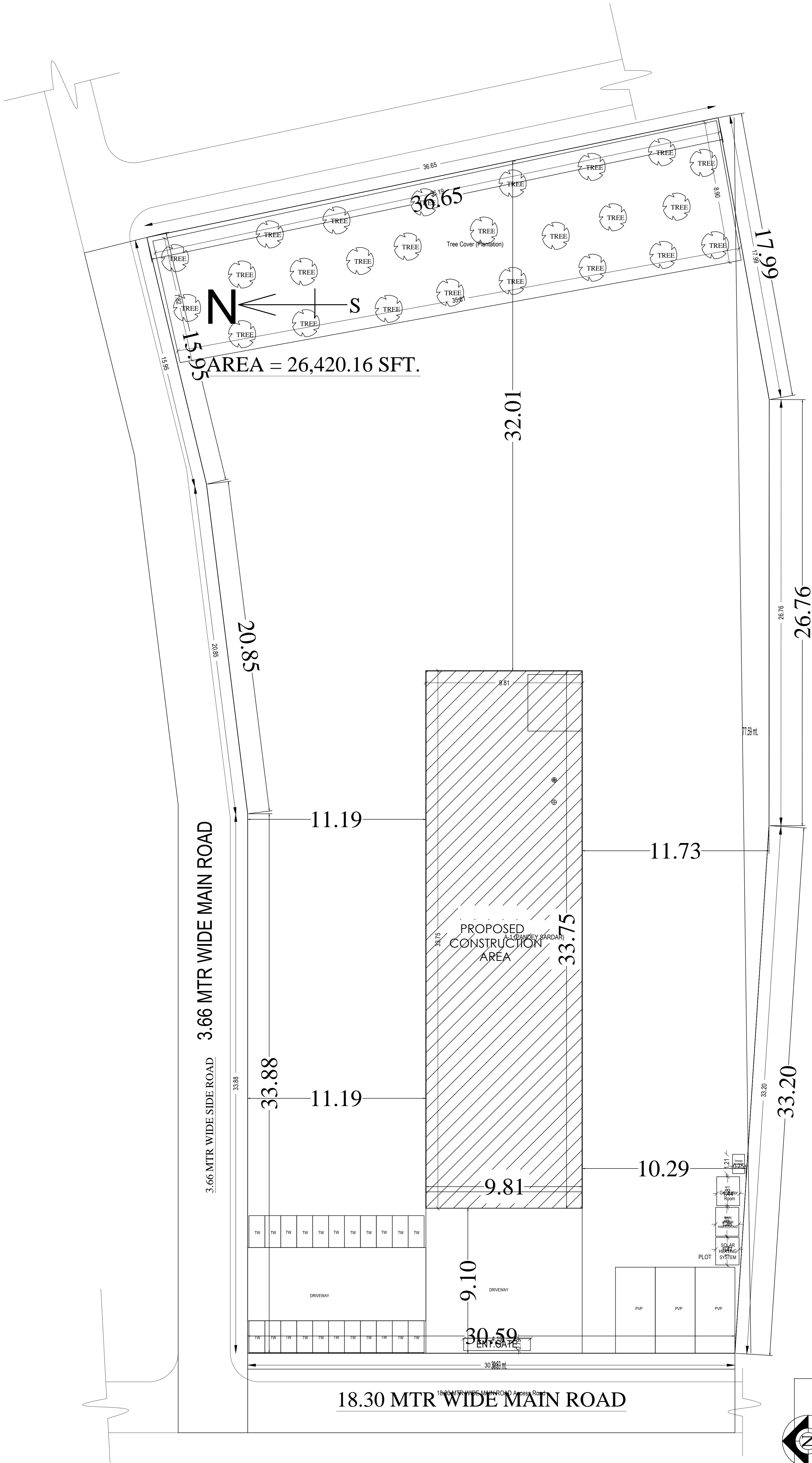
SITE PLAN
