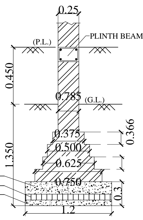
DET. OF WALL FOUND.
