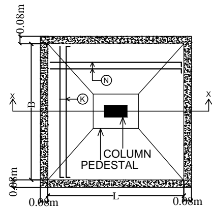
PLAN OF ISOLATED FOOTING
