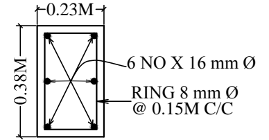
C.S. OF COLUMN SIZE - 0.23M X 0.38M
