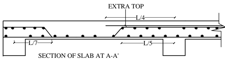
SECTION OF SLAB AT A-A'
