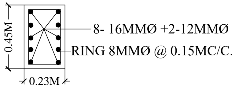
SECTION OF COLUMN.
