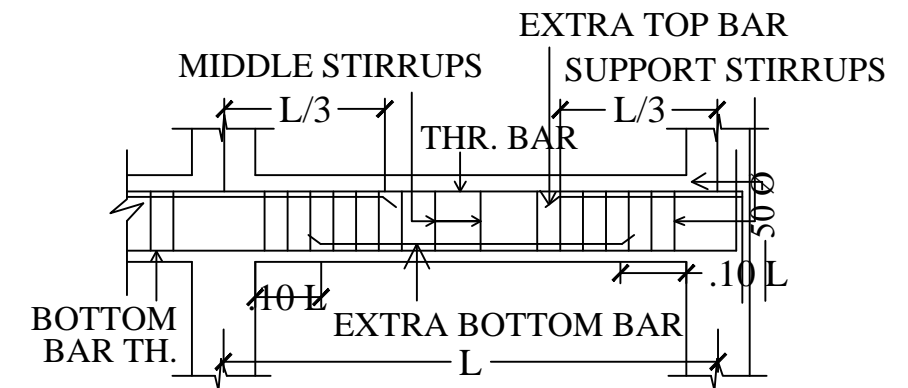
SECTION OF TYPICAL ROOF BEAM
