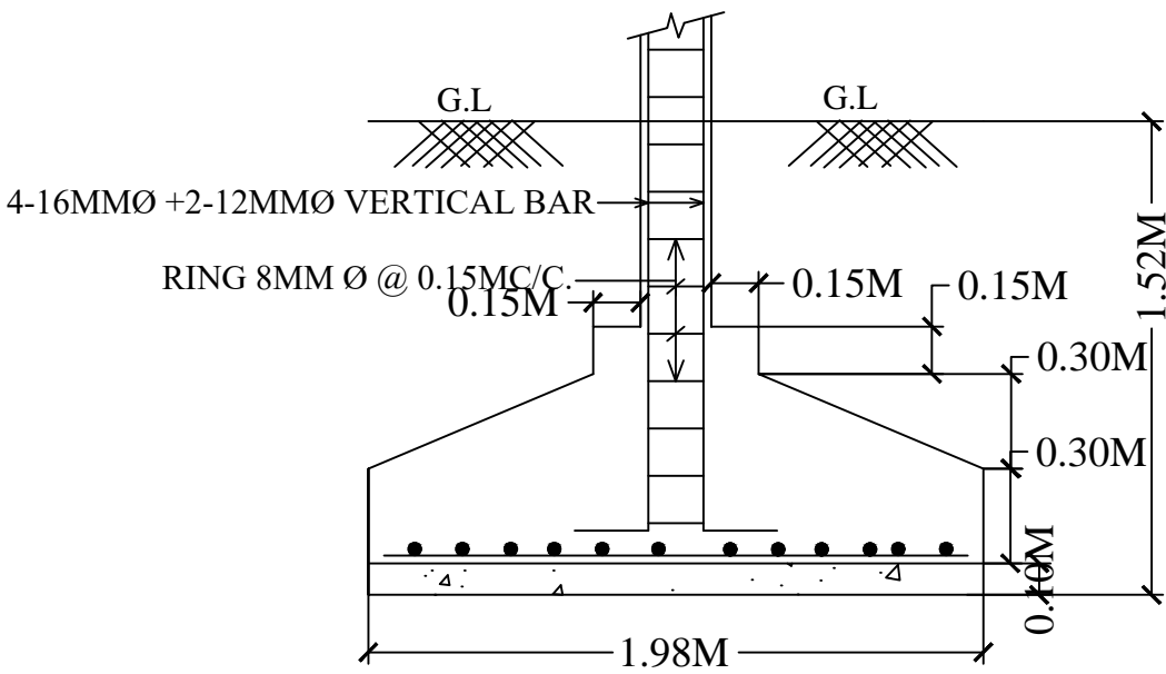
SECTION OF FOOTING
