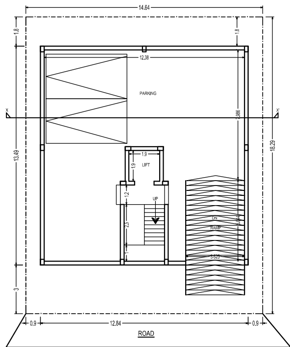
BASEMENT PLAN SCALE: 1:100
