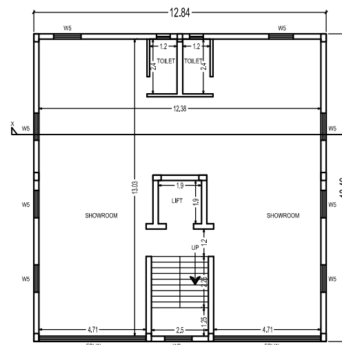
FIRST, SECOND & THIRD FLOOR PLAN SCALE: 1:100
