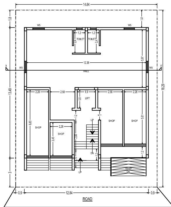
GROUND AND PARKING FLOOR PLAN SCALE: 1:100
