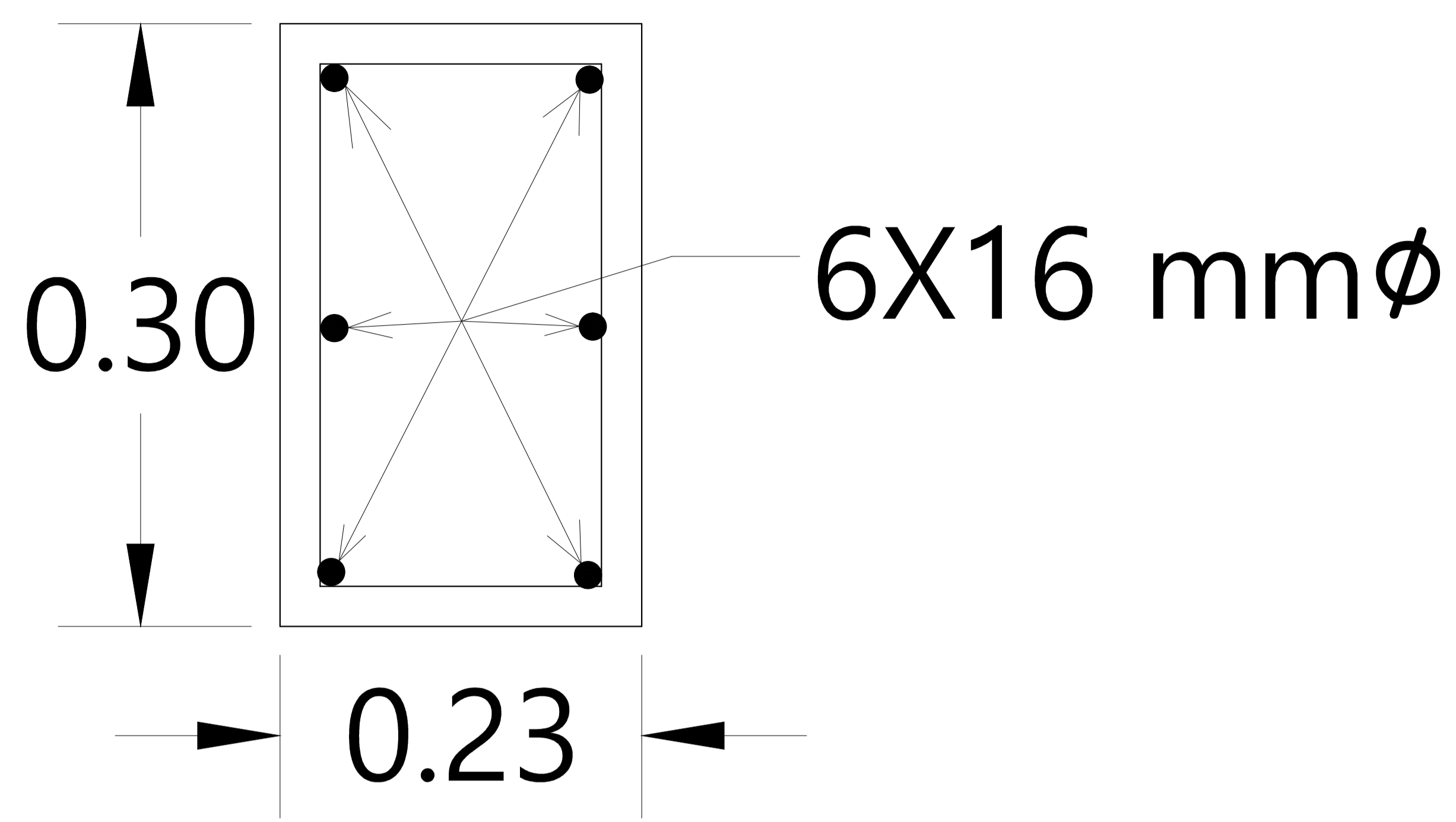
SECTION OF COLUMN
