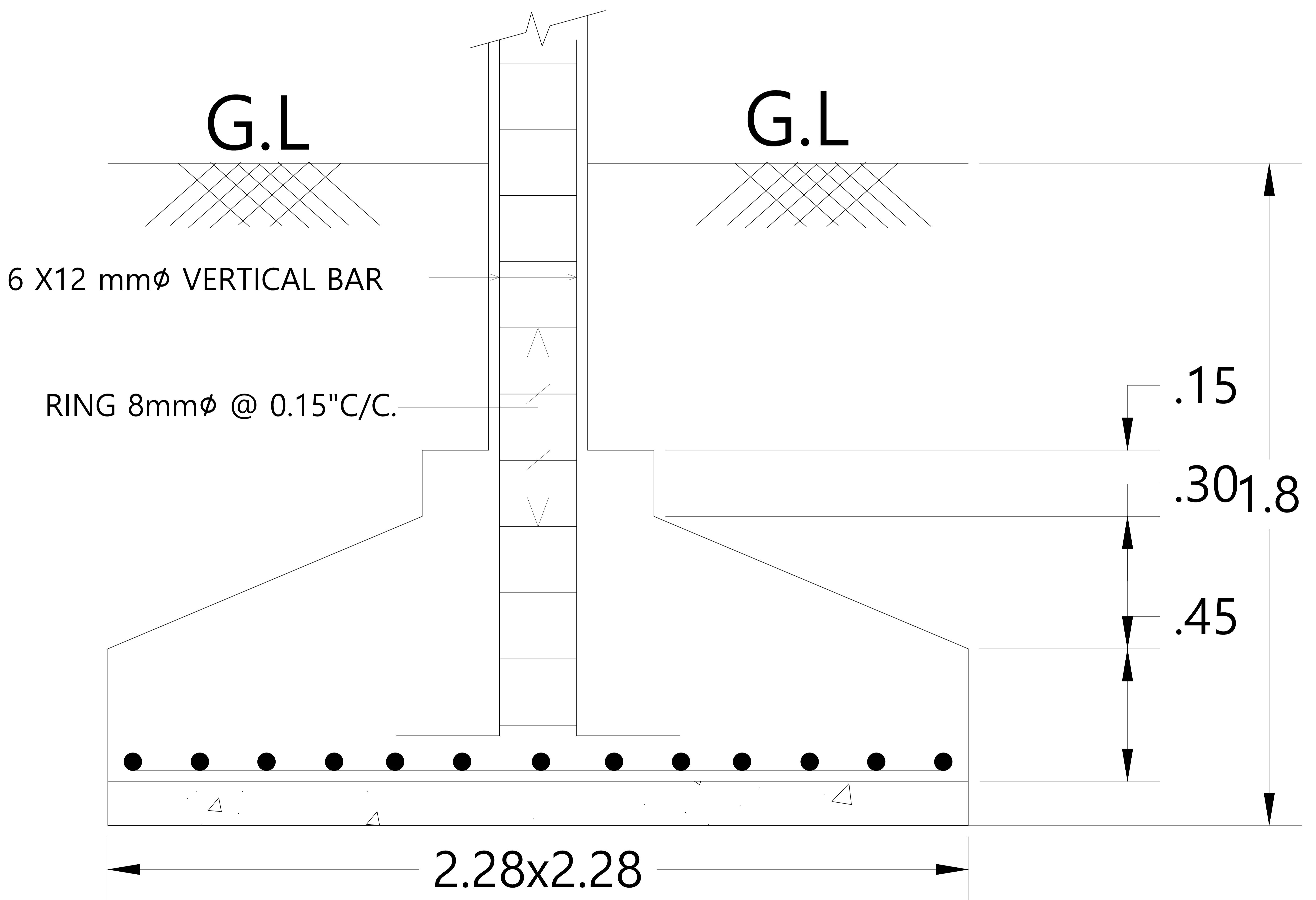
SECTION OF FOOTING
