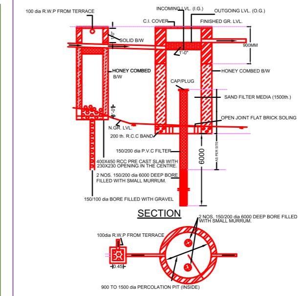
WATER HARVESTING PLAN (NTS)
