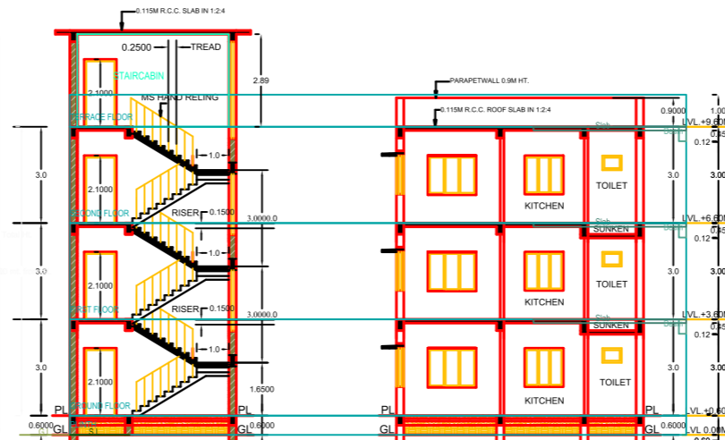
SECTION- AA SECTION- BB SCALE 1:100
