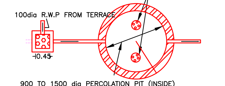
WATER HARVESTING PLAN (NTS)
