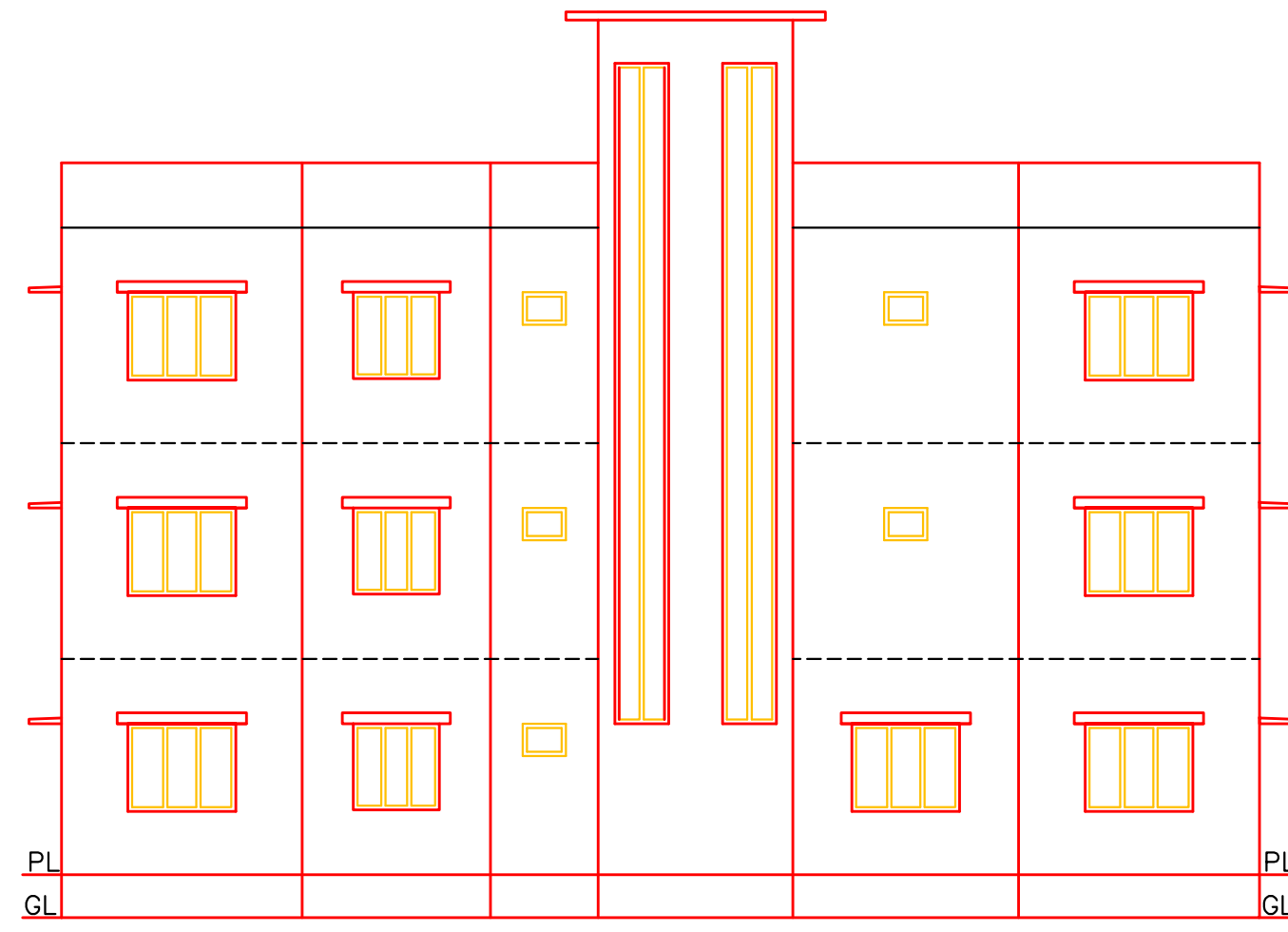
EAST SIDE ELEVATION SCALE 1:100
