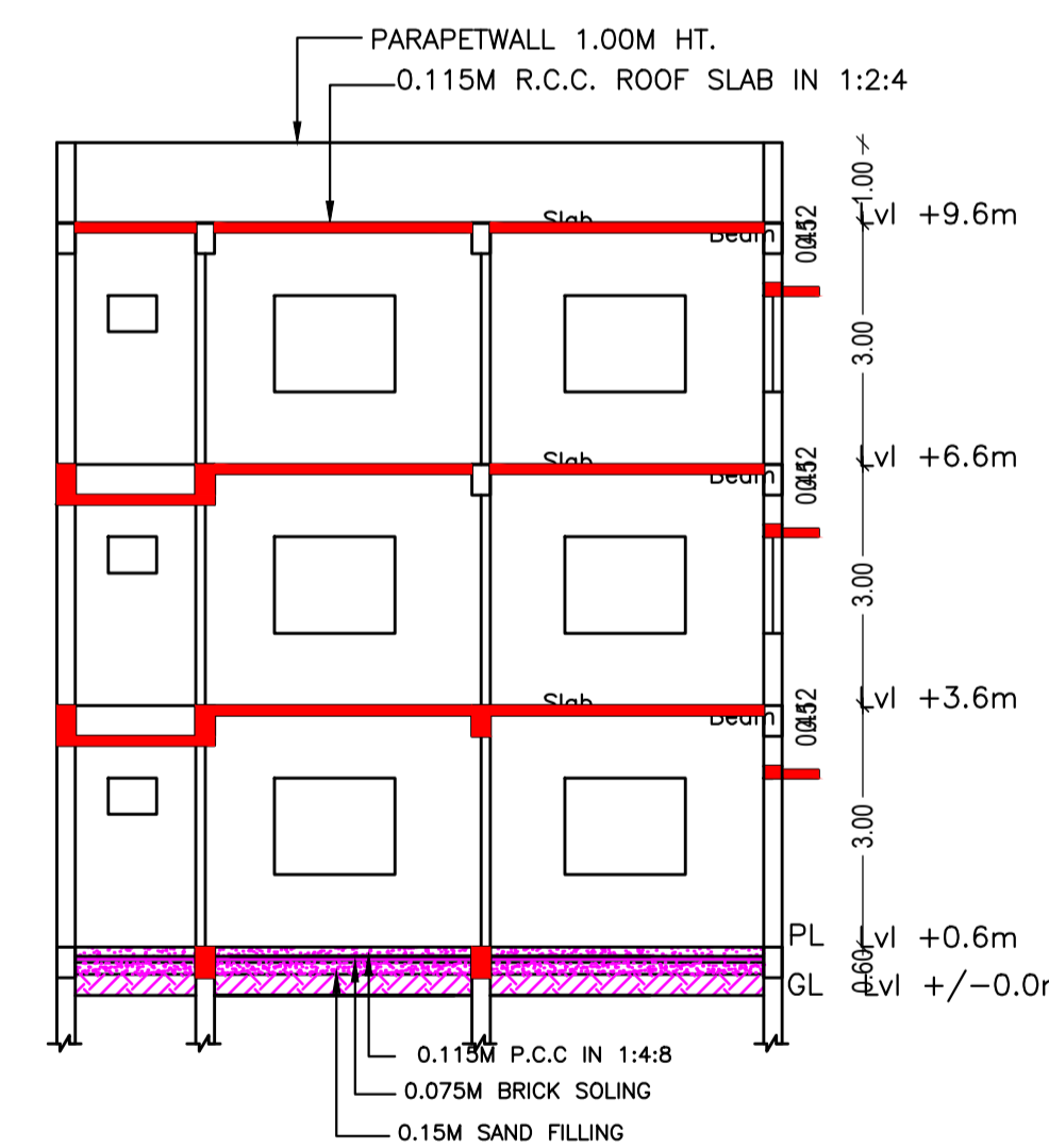
SECTION -B B (SCALE 1:100)
