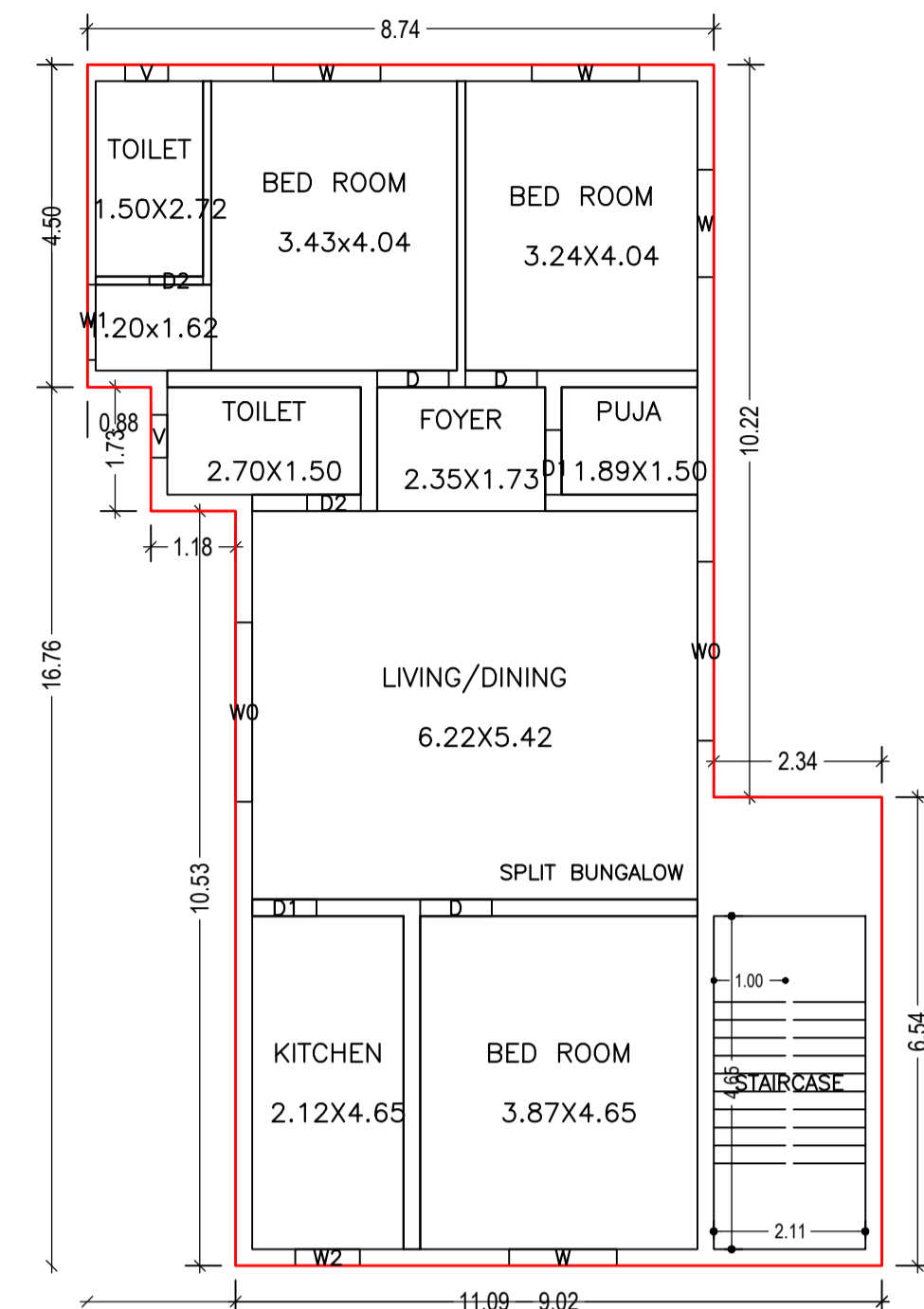
TYPICAL - 1& 2 FLOOR PLAN (Proposed) (SCALE 1:100)
