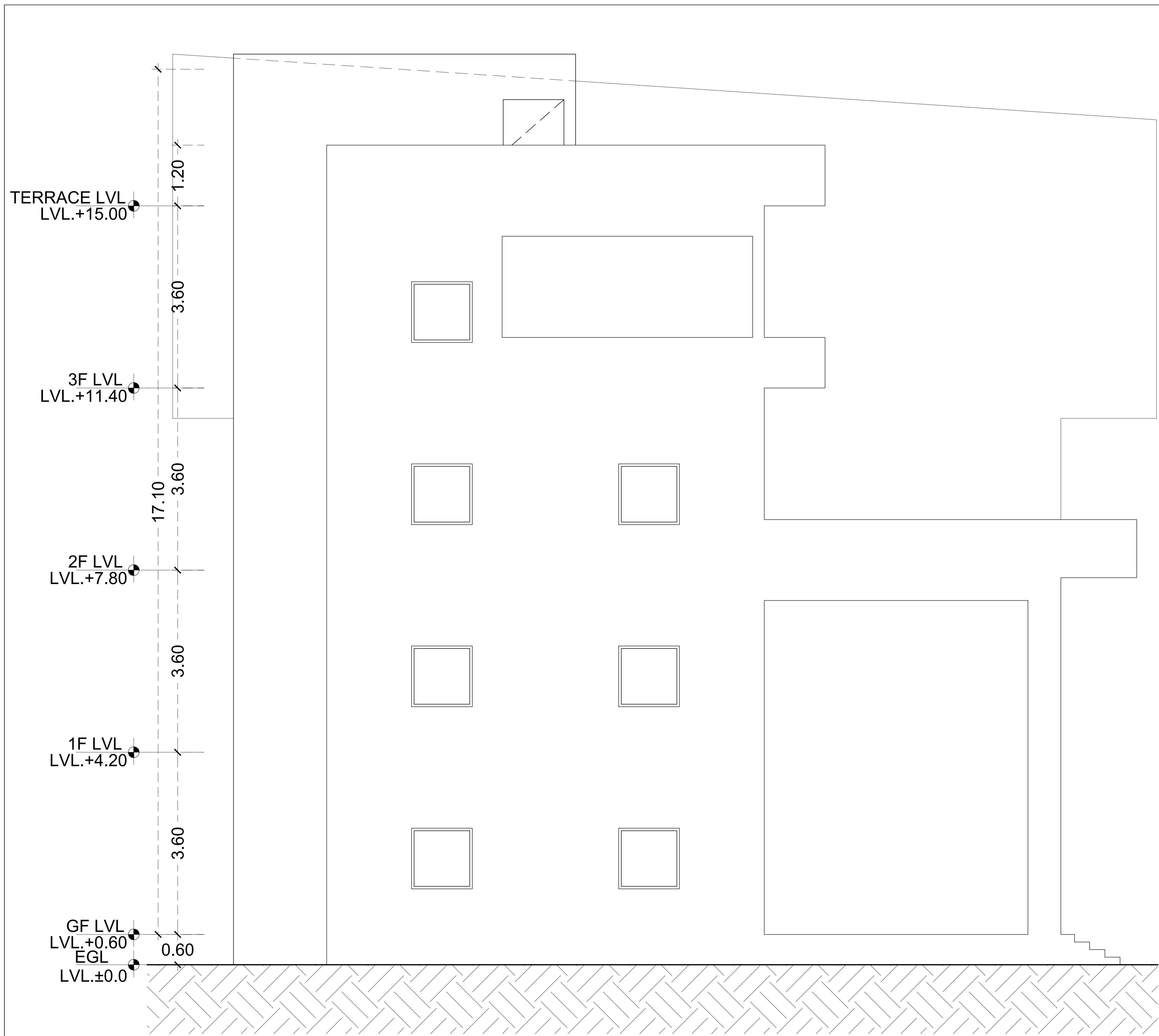
NORTH ELEVATION
