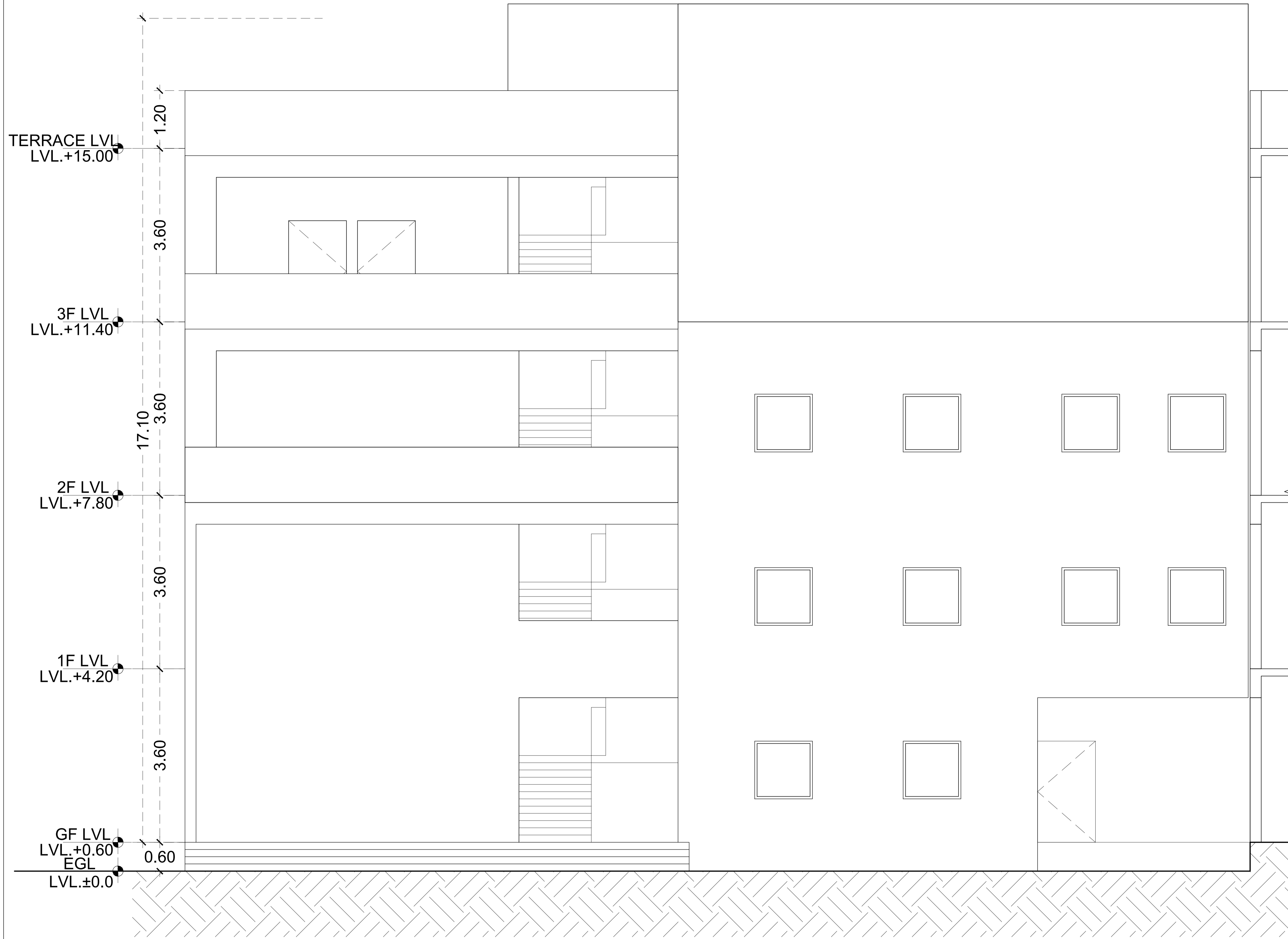
WEST ELEVATION
