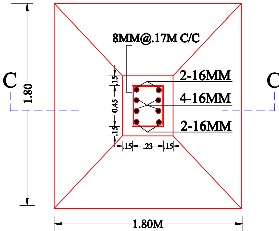
R.C.C. COL. FDN. PLAN SCALE -1:25
