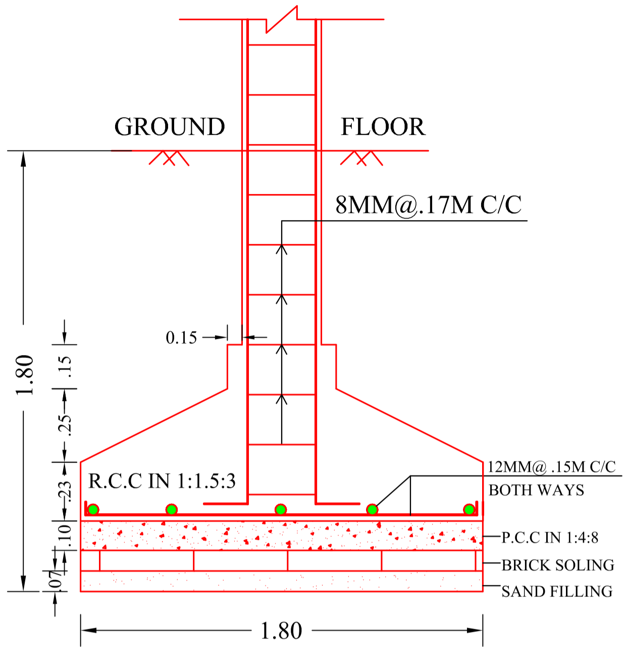
SECTION - CC SCALE -1:25
