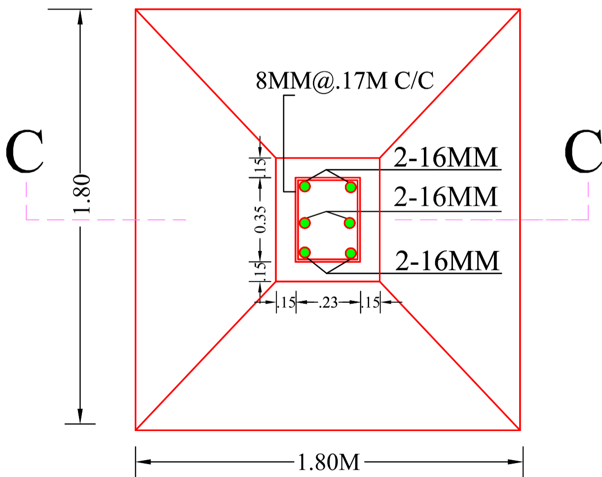
R.C.C. COL. FDN. PLAN SCALE -1:25
