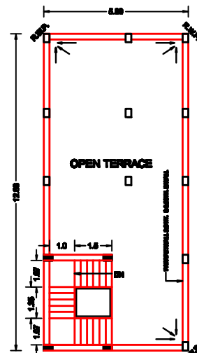
OPEN TERRACE PLAN SCALE 1:100
