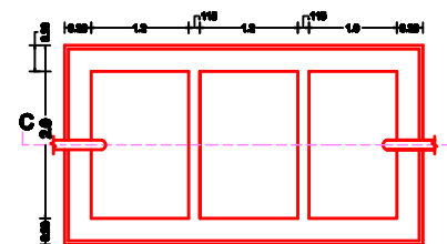
SEPTIC TANK PLAN SCALE 1:100
