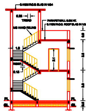
SECTION-AA SCALE 1:100
