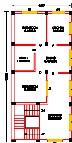
FIRST FLOOR PLAN SCALE 1:100
