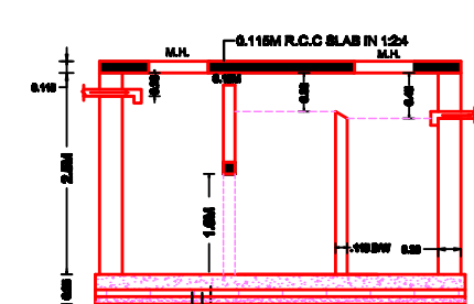
SECTION-SS SCALE 1:100
