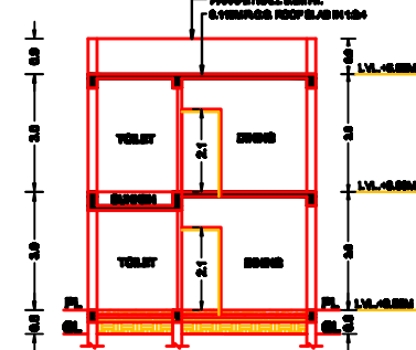
SECTION-BB SCALE 1:100
