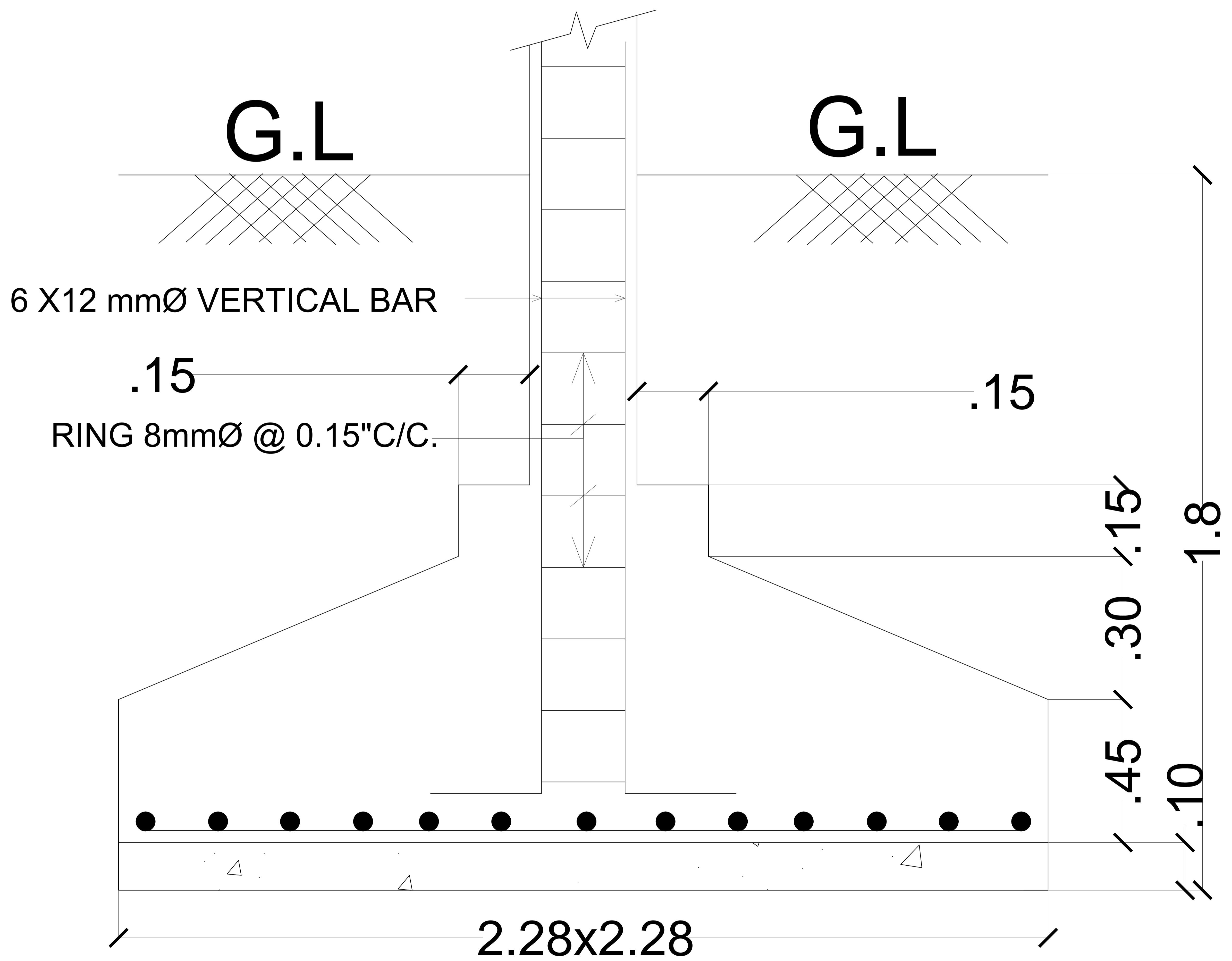
SECTION OF FOOTING
