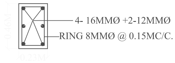
SECTION OF COLUMN.
