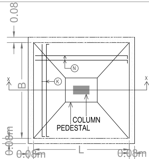
PLAN OF ISOLATED FOOTING
