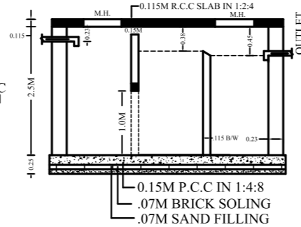
SECTION - SS SCALE -1:50
