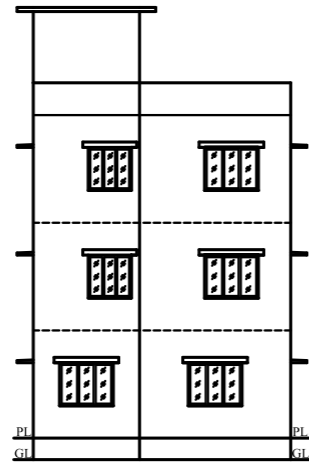
NORTH SIDE ELEVATION SCALE 1:100
