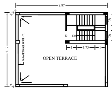
OPEN TERRACE PLAN SCALE 1:100
