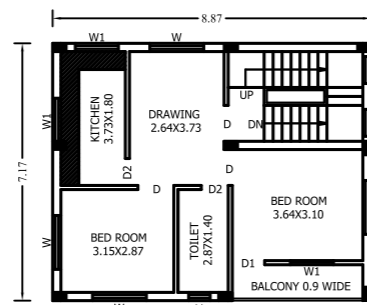
1ST & 2ND FLOOR PLAN SCALE 1:100
