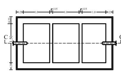
SEPTIC TANK PLAN SCALE -1:50
