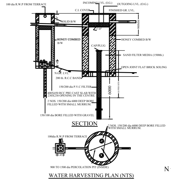
WATER HARVESTING PLAN (NTS)
