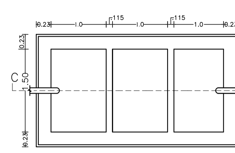
SEPTIC TANK PLAN SCALE -1:50
