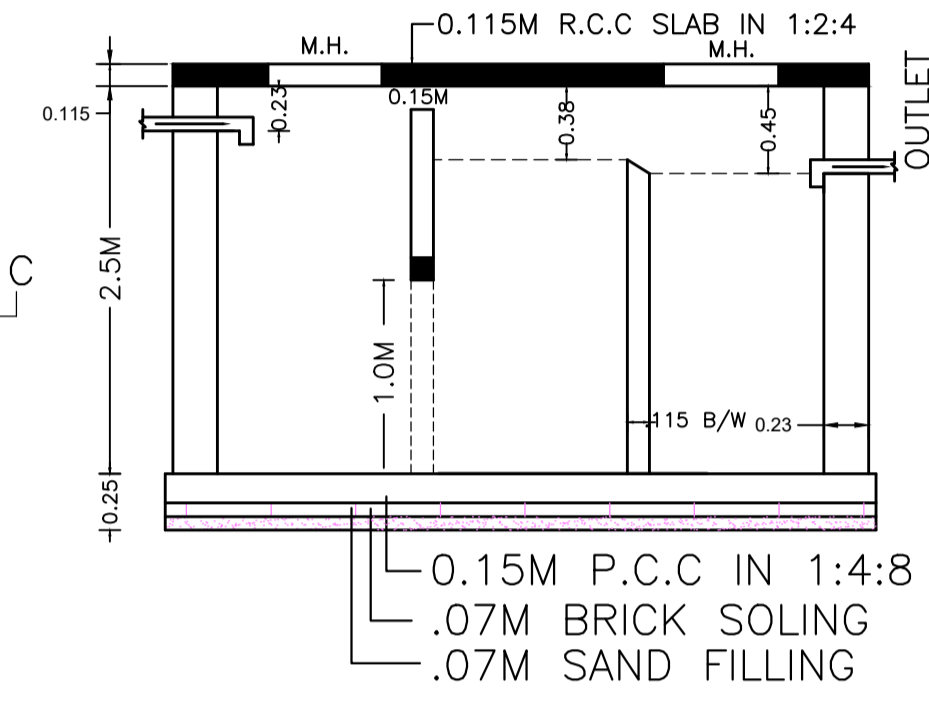
SECTION - SS SCALE -1:50
