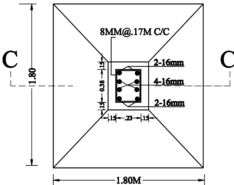
R.C.C. COL. FDN. PLAN SCALE -1:25
