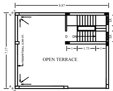
OPEN TERRACE PLAN SCALE 1:100
