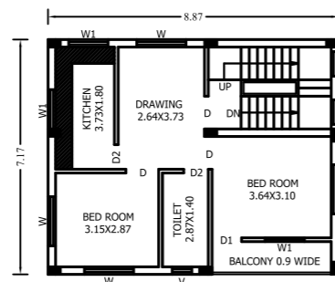
1ST & 2ND FLOOR PLAN SCALE 1:100
