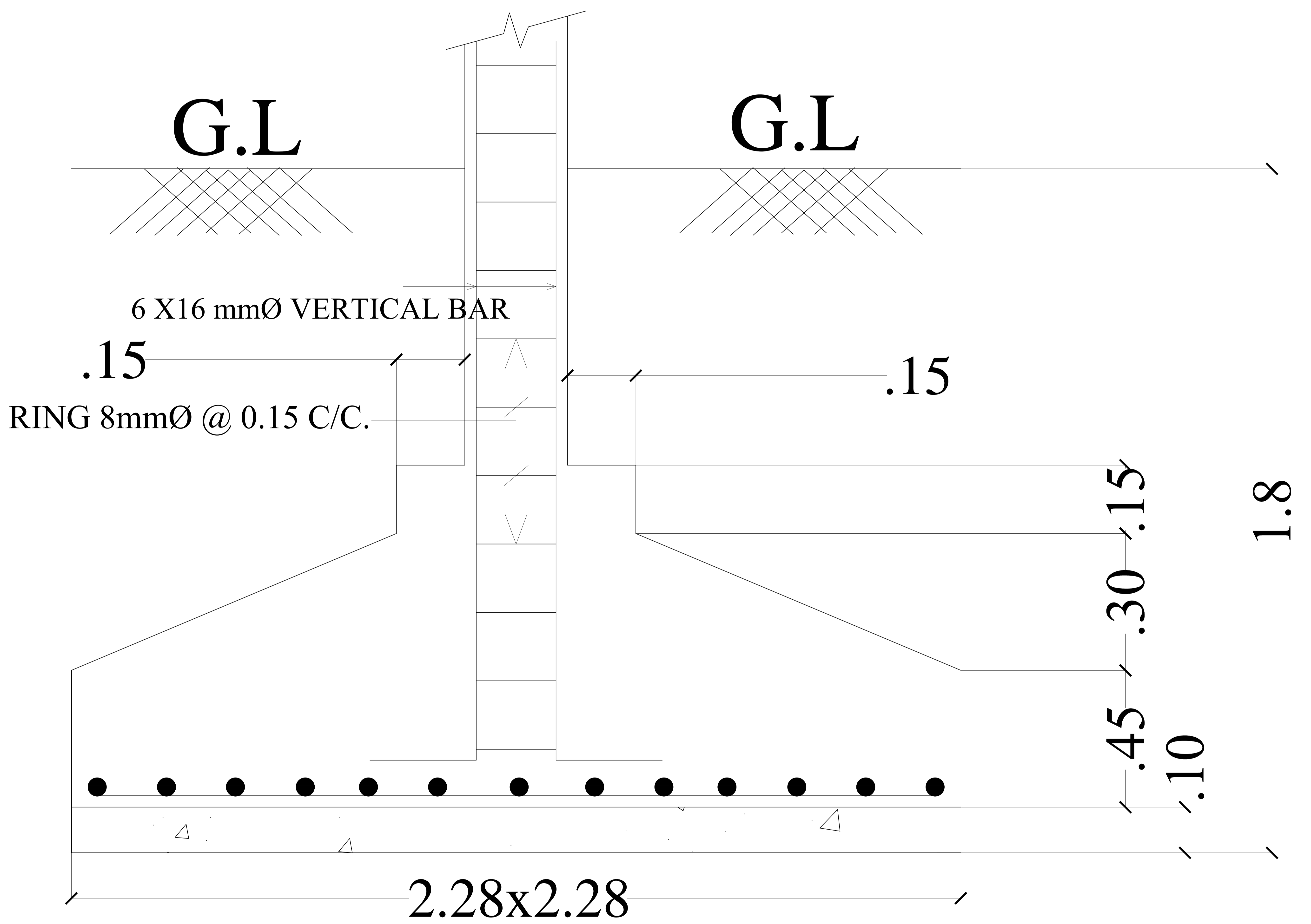
SECTION OF FOOTING
