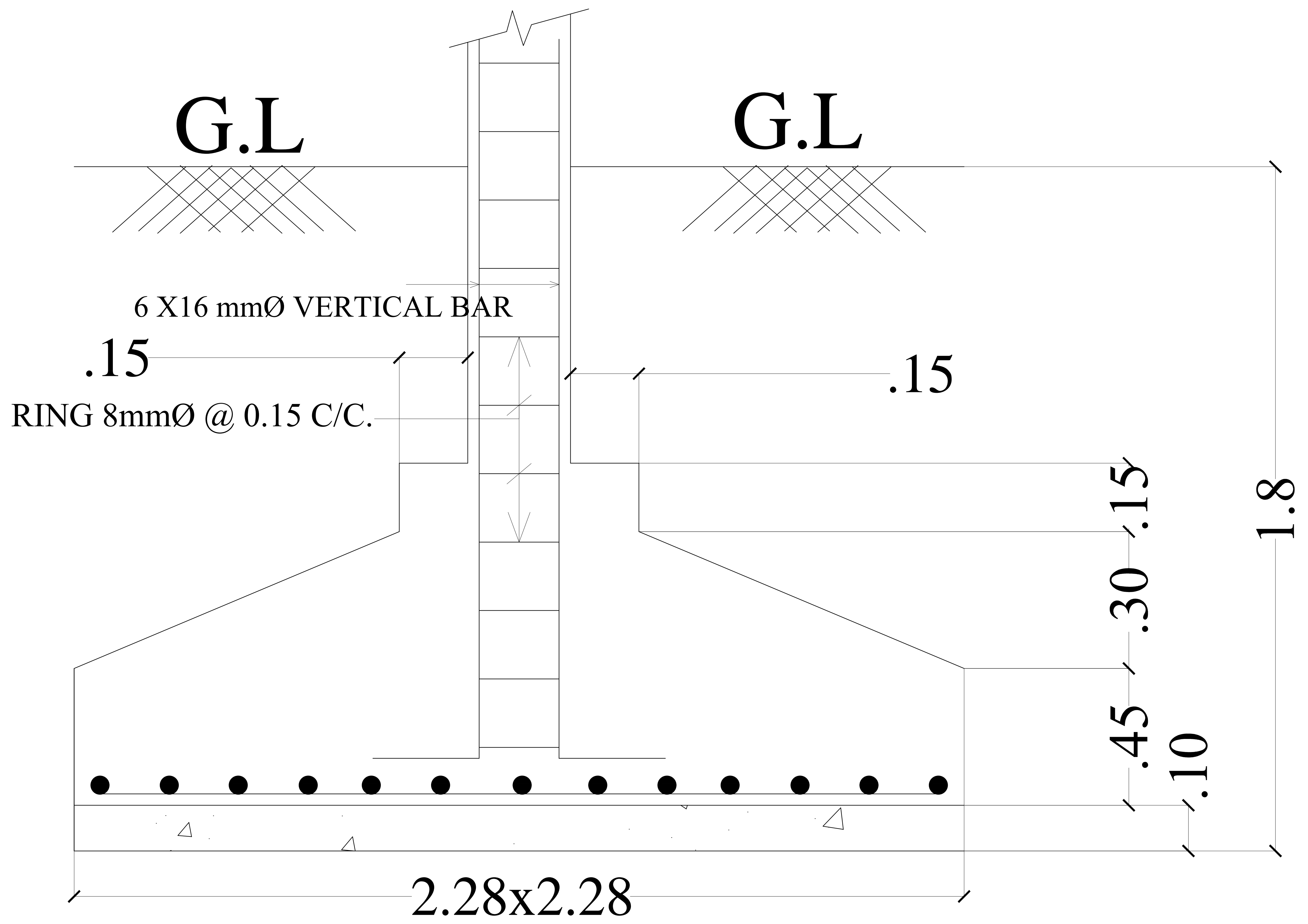
SECTION OF FOOTING
