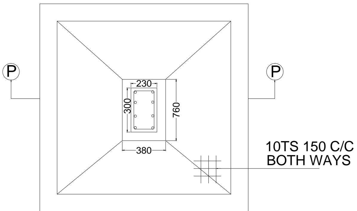
PLAN FOOTING PLAN (AS/STRL. DESIGN) SCALE N.T.S
